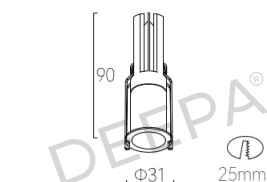
DP-RMSA-ER5/6 Fixed
