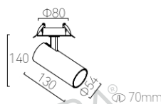
DP-TSRP-OP12(R) Recessed
